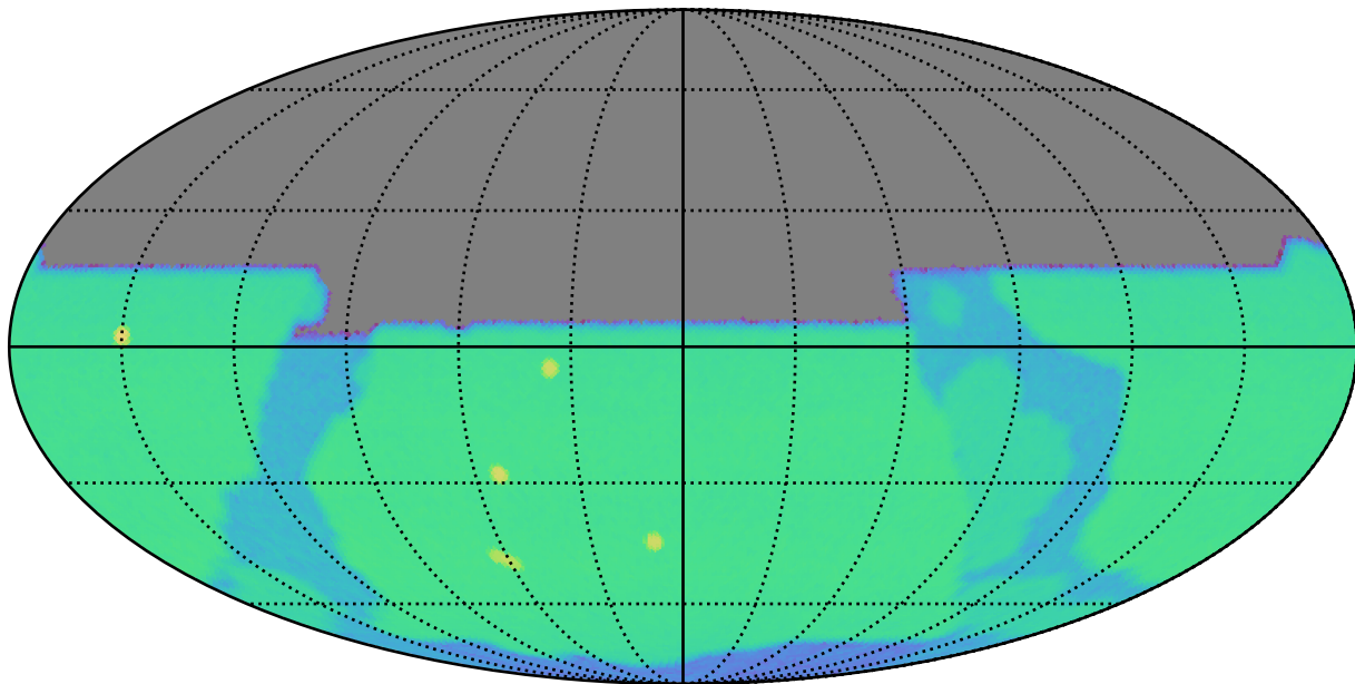
too_5_4v3.4_10yrs y: SurfaceBrightLimit
