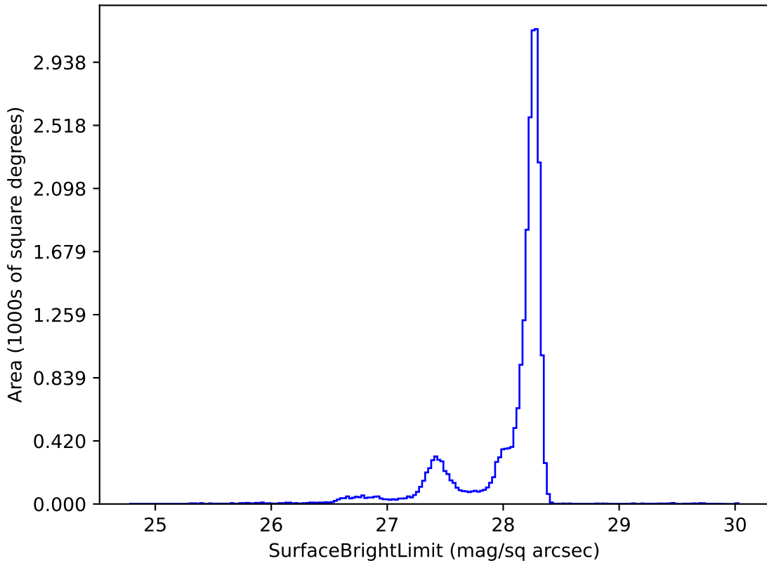
too_5_4v3.4_10yrs y: SurfaceBrightLimit
