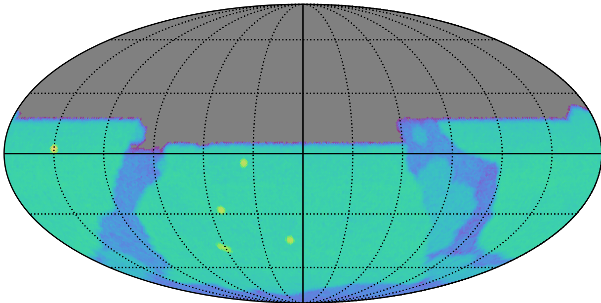
too_5_4v3.4_10yrs u: SurfaceBrightLimit
