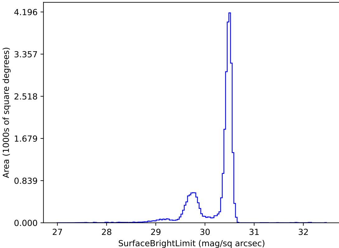
too_5_4v3.4_10yrs r: SurfaceBrightLimit
