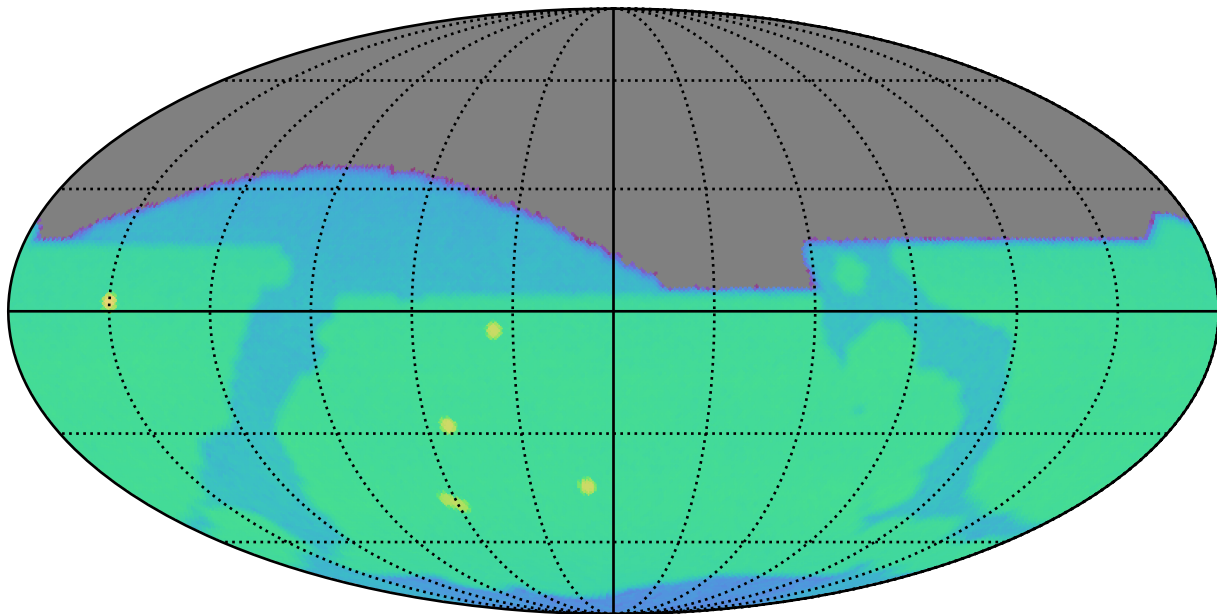
too_5_4v3.4_10yrs i: SurfaceBrightLimit
