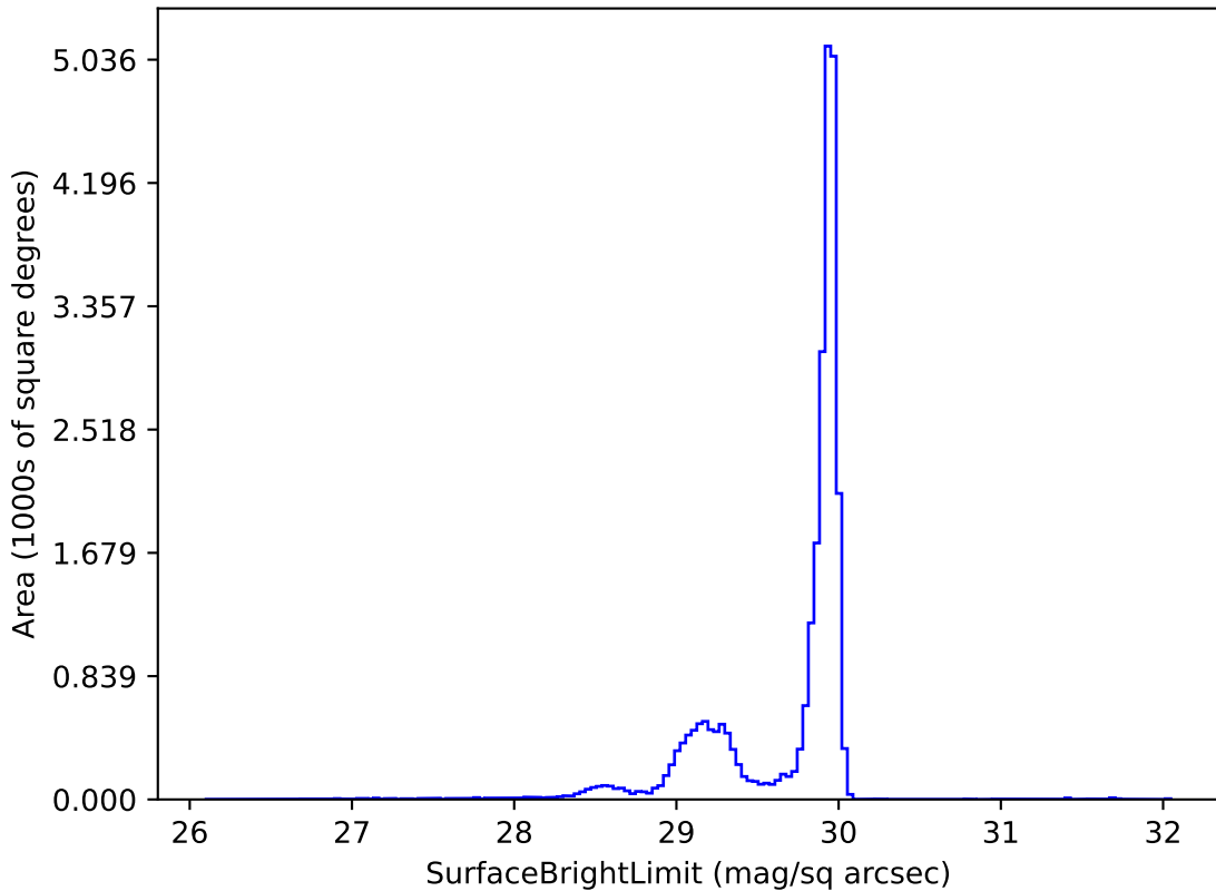
too_5_4v3.4_10yrs i: SurfaceBrightLimit
