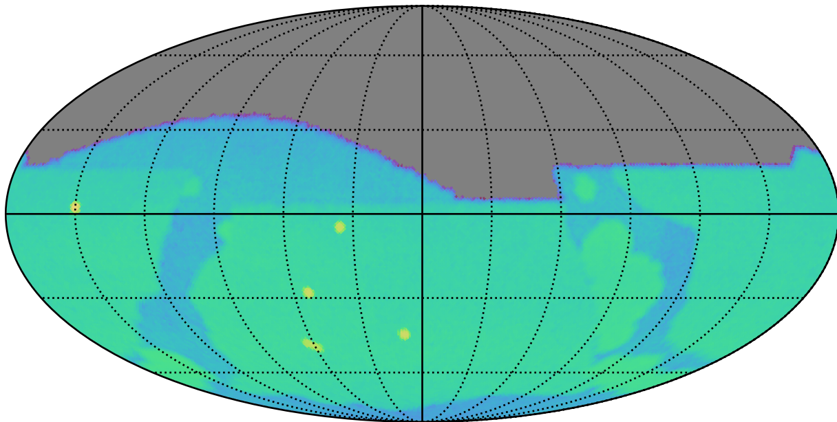
too_5_4v3.4_10yrs g: SurfaceBrightLimit
