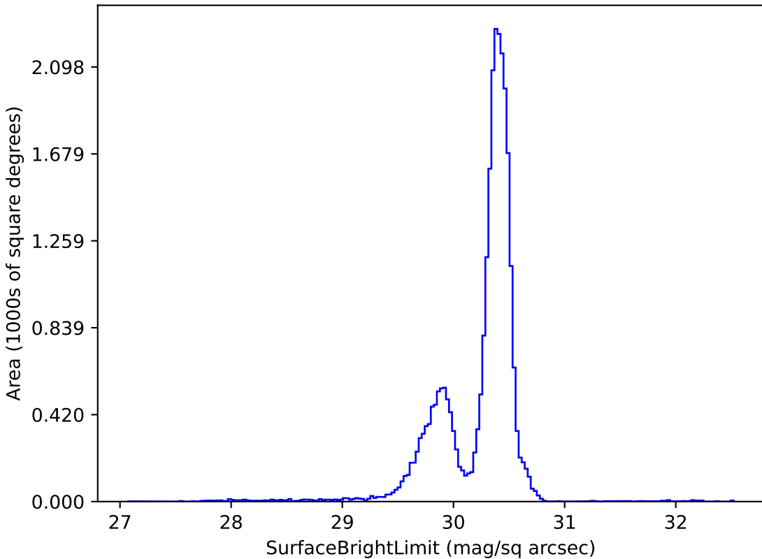
too_5_4v3.4_10yrs g: SurfaceBrightLimit
