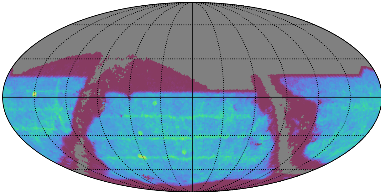
too_5_4v3.4_10yrs : SNSLMetric
