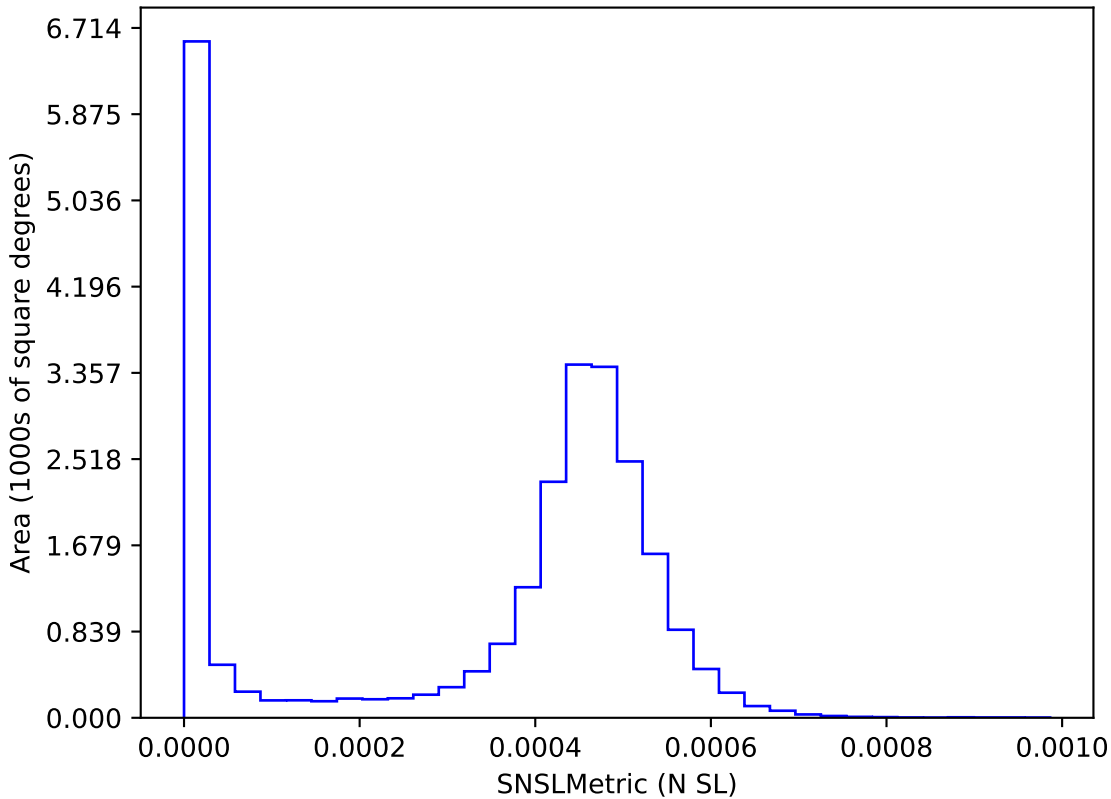
too_5_4v3.4_10yrs : SNSLMetric
