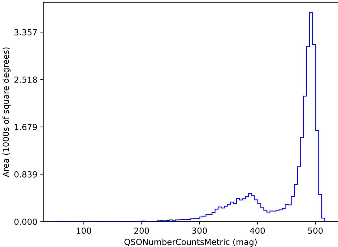
too_5_4v3.4_10yrs z band and non-DD: QSONumberCountsMetric
