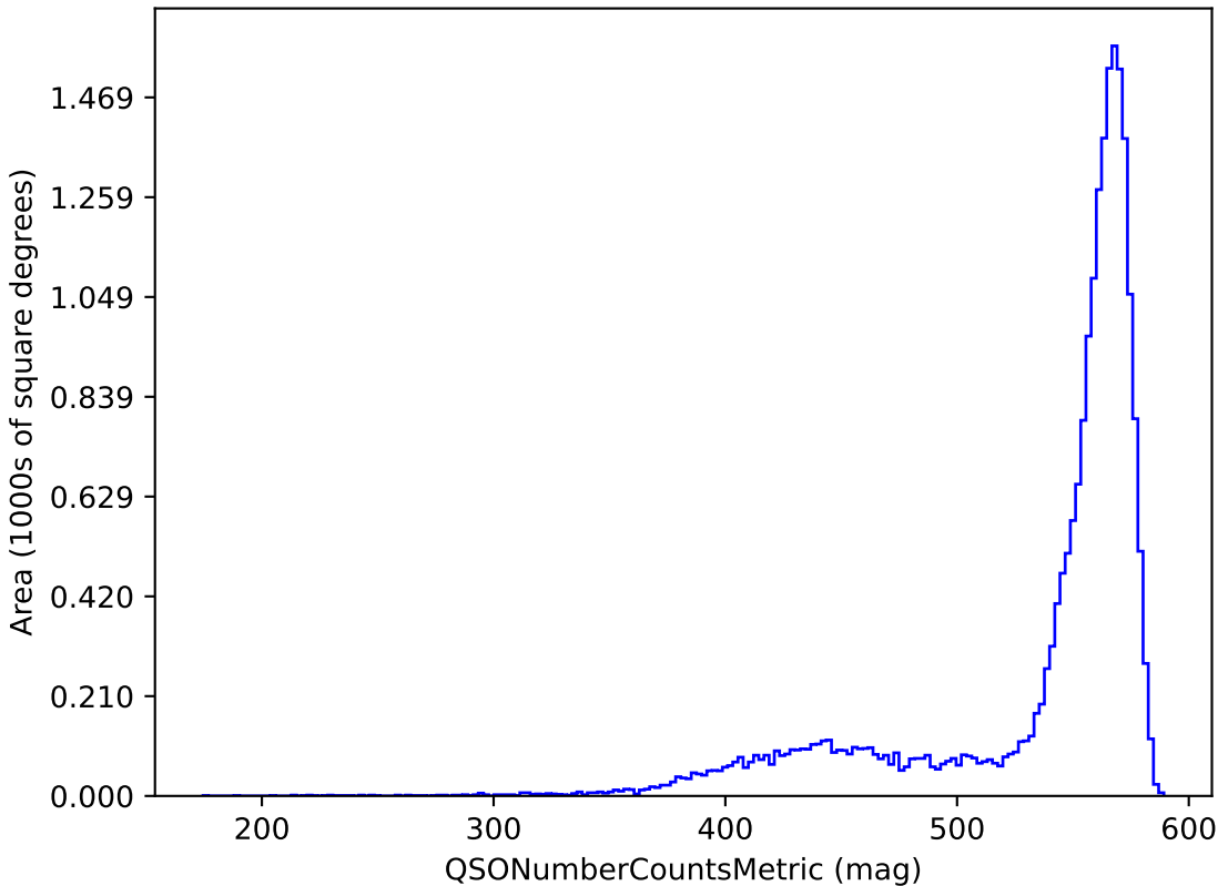
too_5_4v3.4_10yrs y band and non-DD: QSONumberCountsMetric
