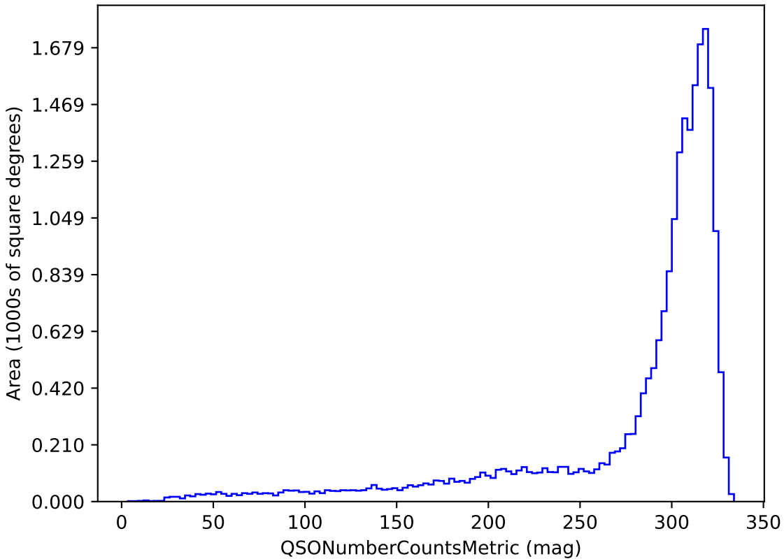
too_5_4v3.4_10yrs u band and non-DD: QSONumberCountsMetric
