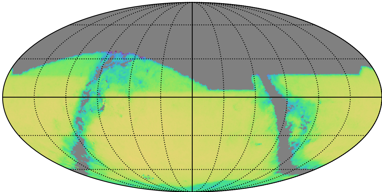
too_5_4v3.4_10yrs r band and non-DD: QSONumberCountsMetric
