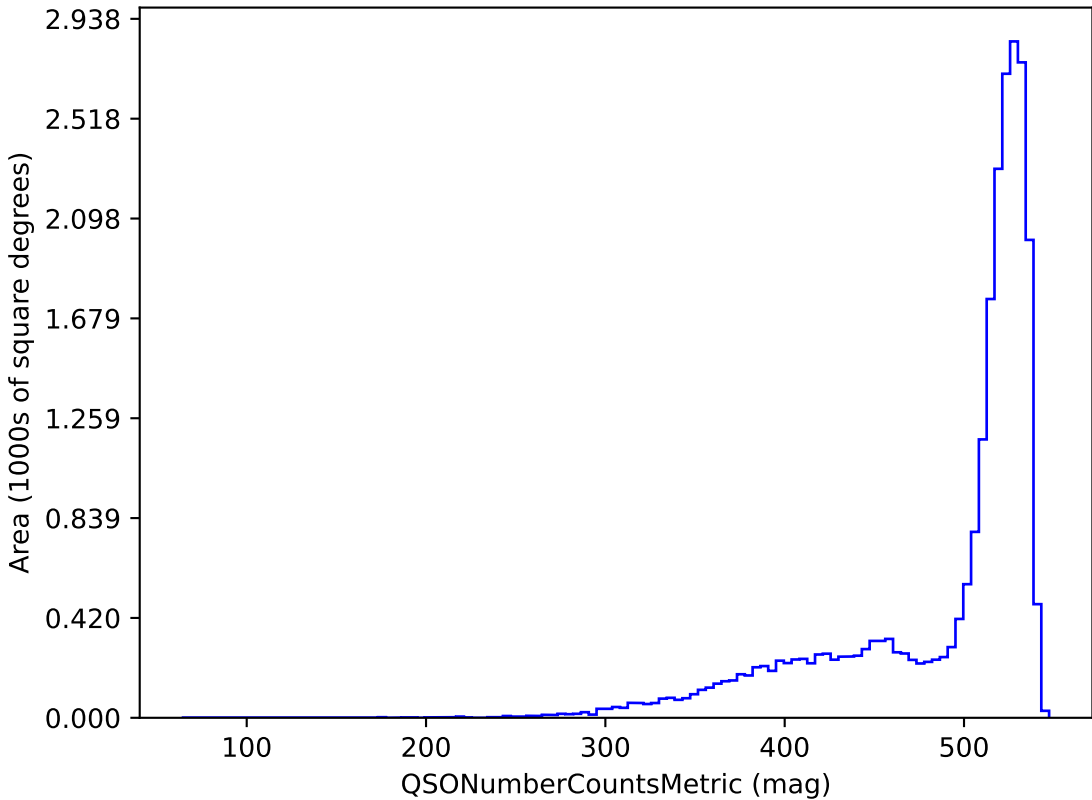
too_5_4v3.4_10yrs r band and non-DD: QSONumberCountsMetric
