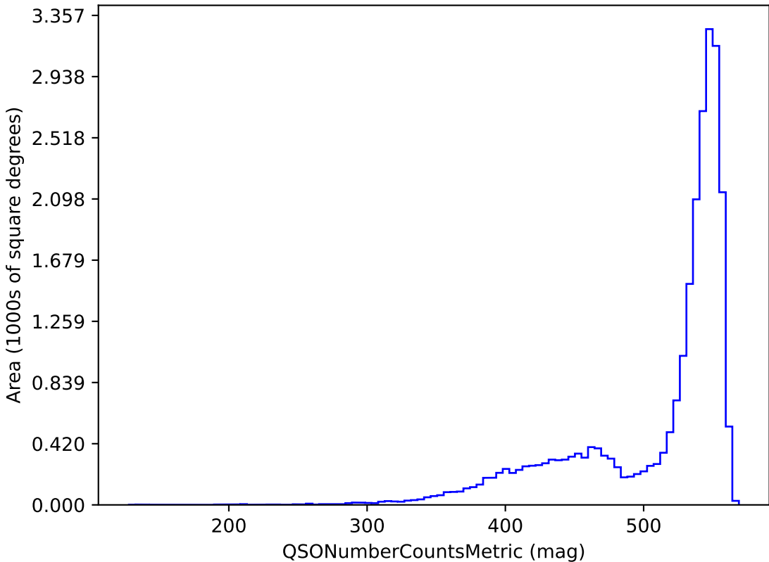
too_5_4v3.4_10yrs i band and non-DD: QSONumberCountsMetric
