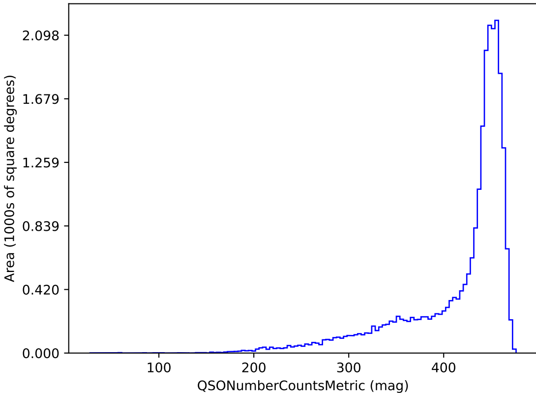
too_5_4v3.4_10yrs g band and non-DD: QSONumberCountsMetric
