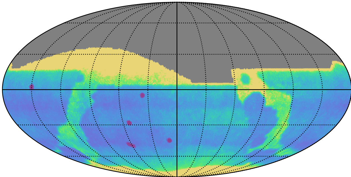
too_5_4v3.4_10yrs : Proper Motion Uncert @ 24.0
