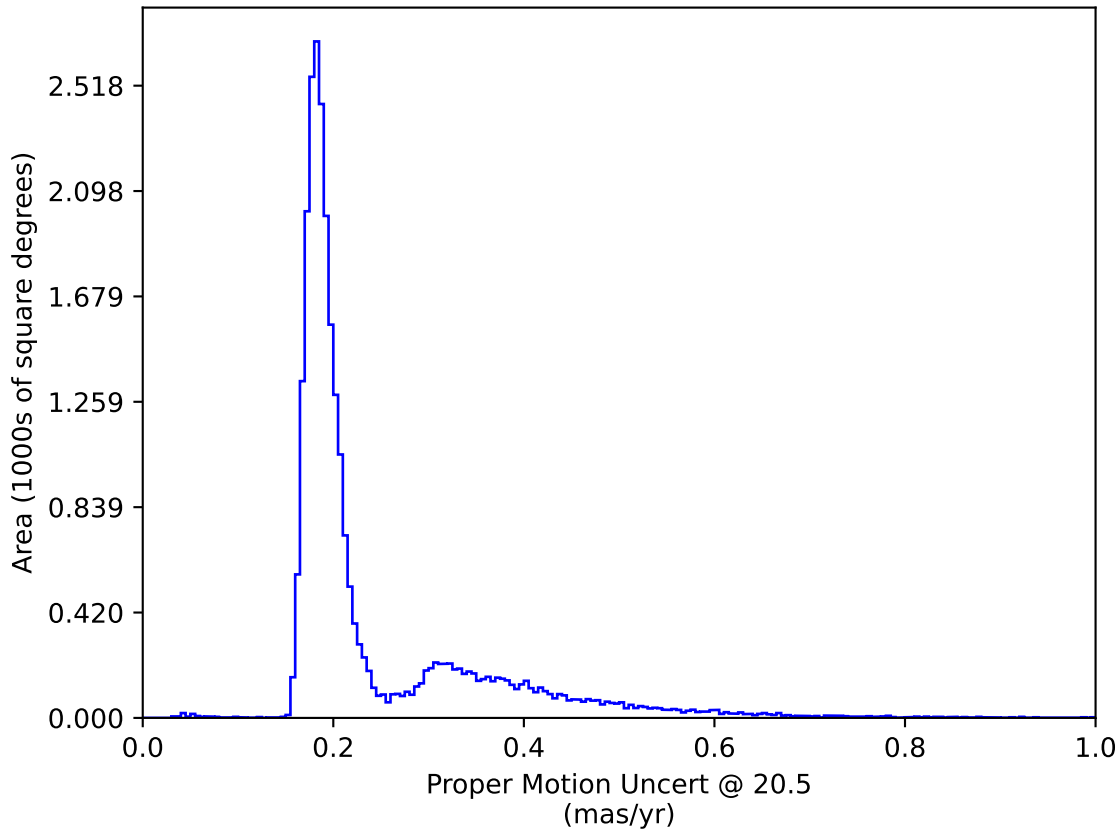
too_5_4v3.4_10yrs : Proper Motion Uncert @ 20.5
