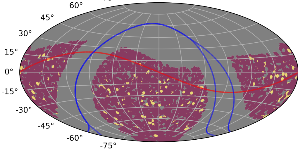
too_5_4v3.4_10yrs : PrestoKNe_score_s 75°
