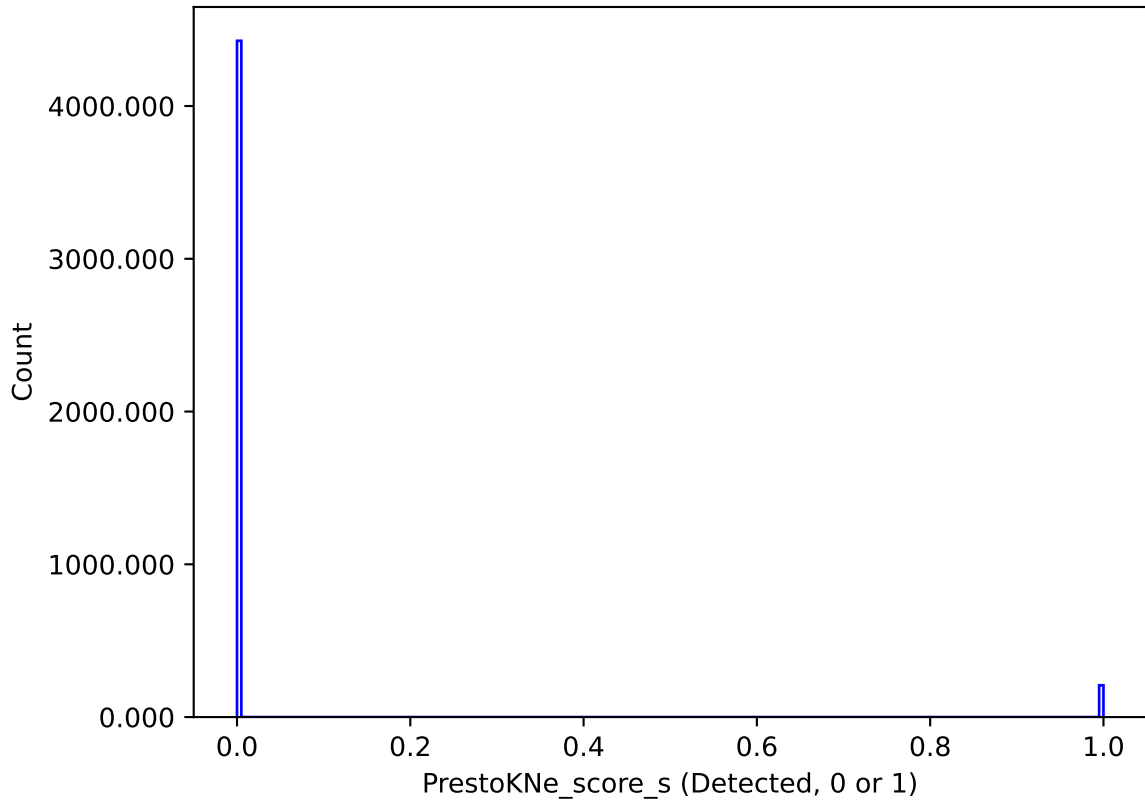
too_5_4v3.4_10yrs : PrestoKNe_score_s
