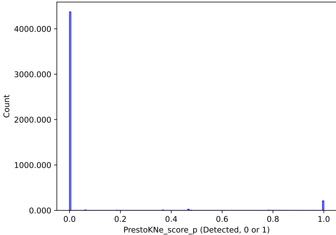
too_5_4v3.4_10yrs : PrestoKNe_score_p
