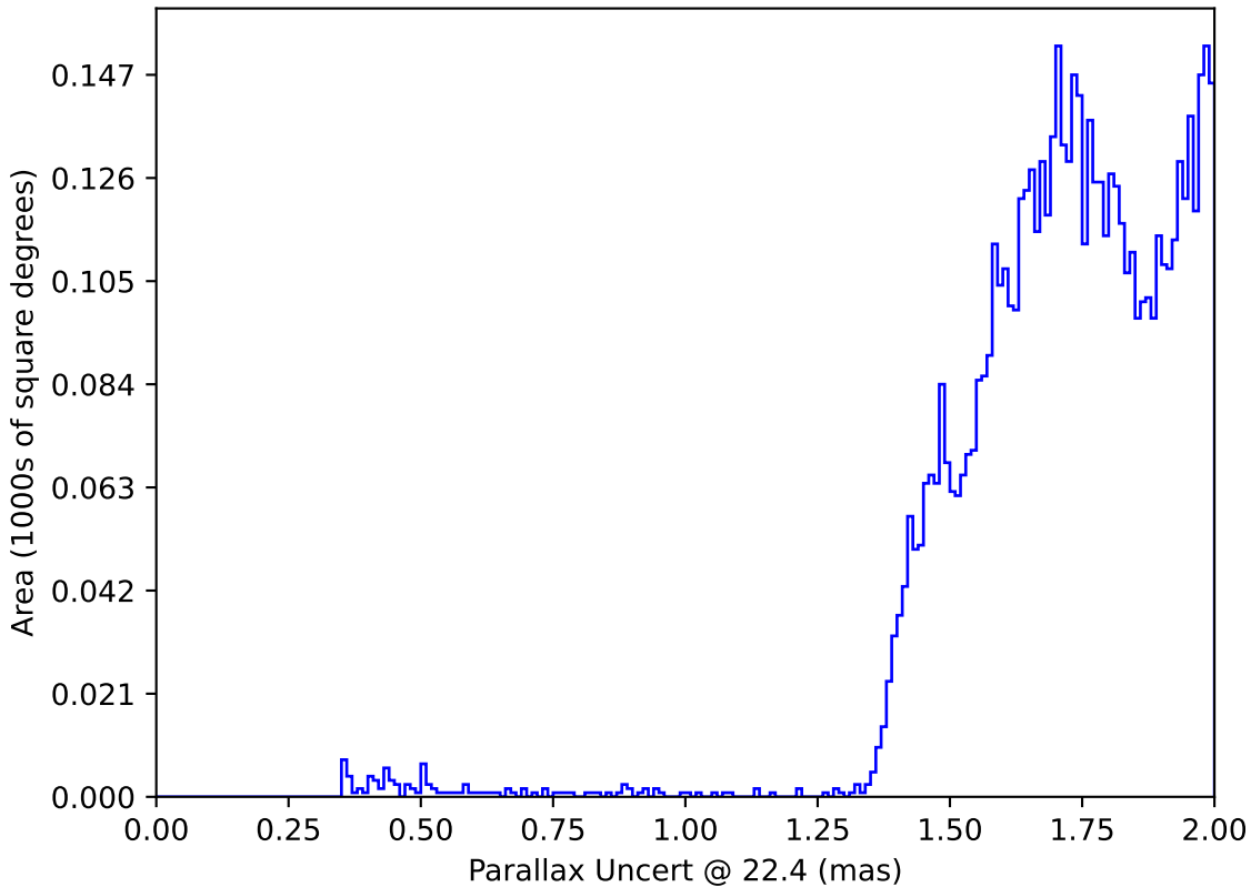
too_5_4v3.4_10yrs : Parallax Uncert @ 22.4
