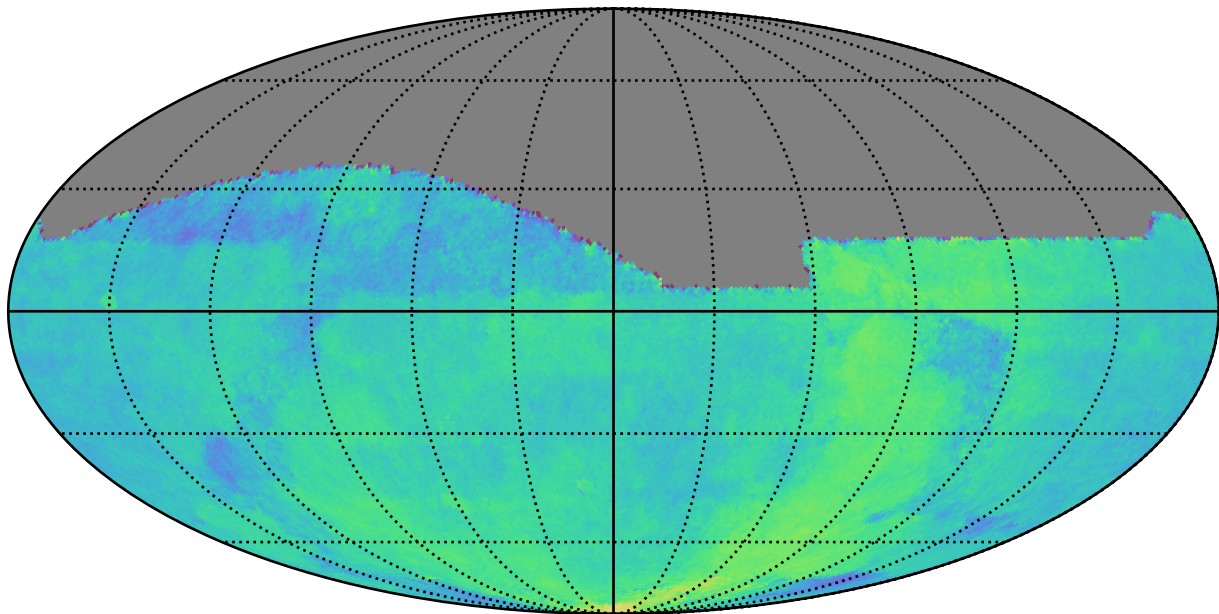
too_5_4v3.4_10yrs : Parallax Coverage @ 24.0
