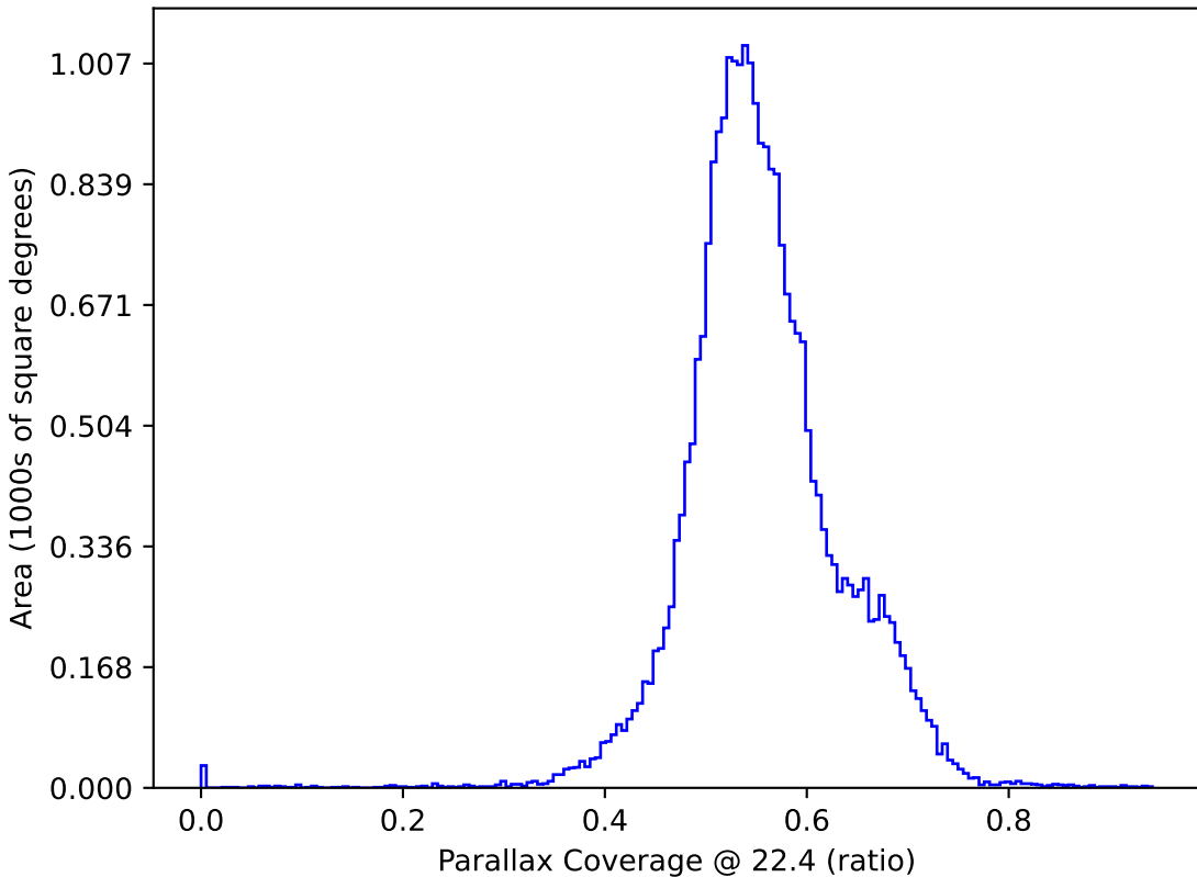
too_5_4v3.4_10yrs : Parallax Coverage @ 22.4
