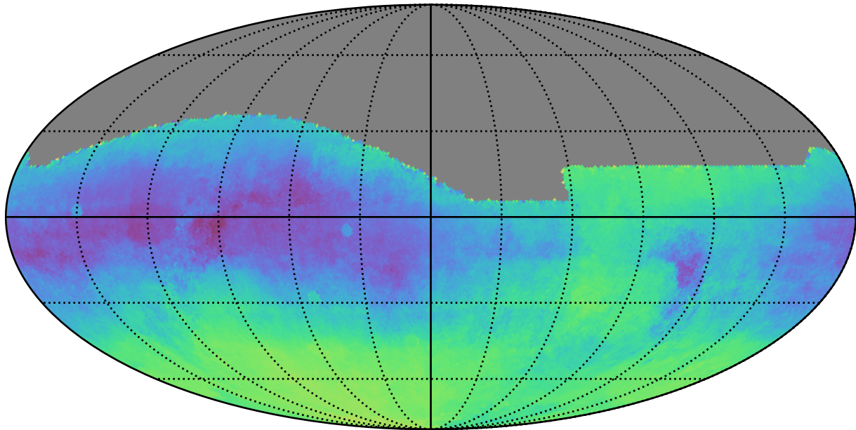
too_5_4v3.4_10yrs : Parallax-DCR degeneracy @ 24.0
