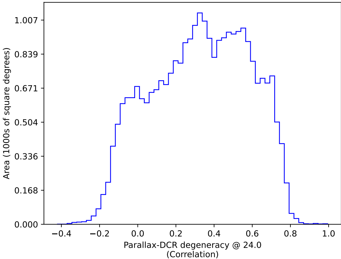
too_5_4v3.4_10yrs : Parallax-DCR degeneracy @ 24.0
