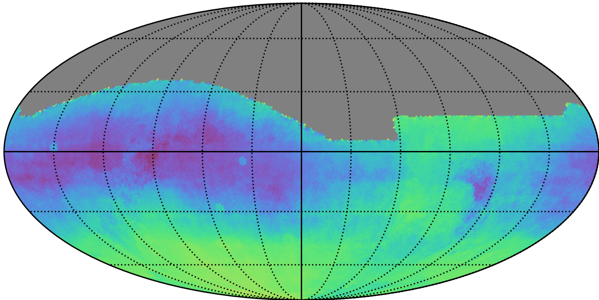
too_5_4v3.4_10yrs : Parallax-DCR degeneracy @ 22.4
