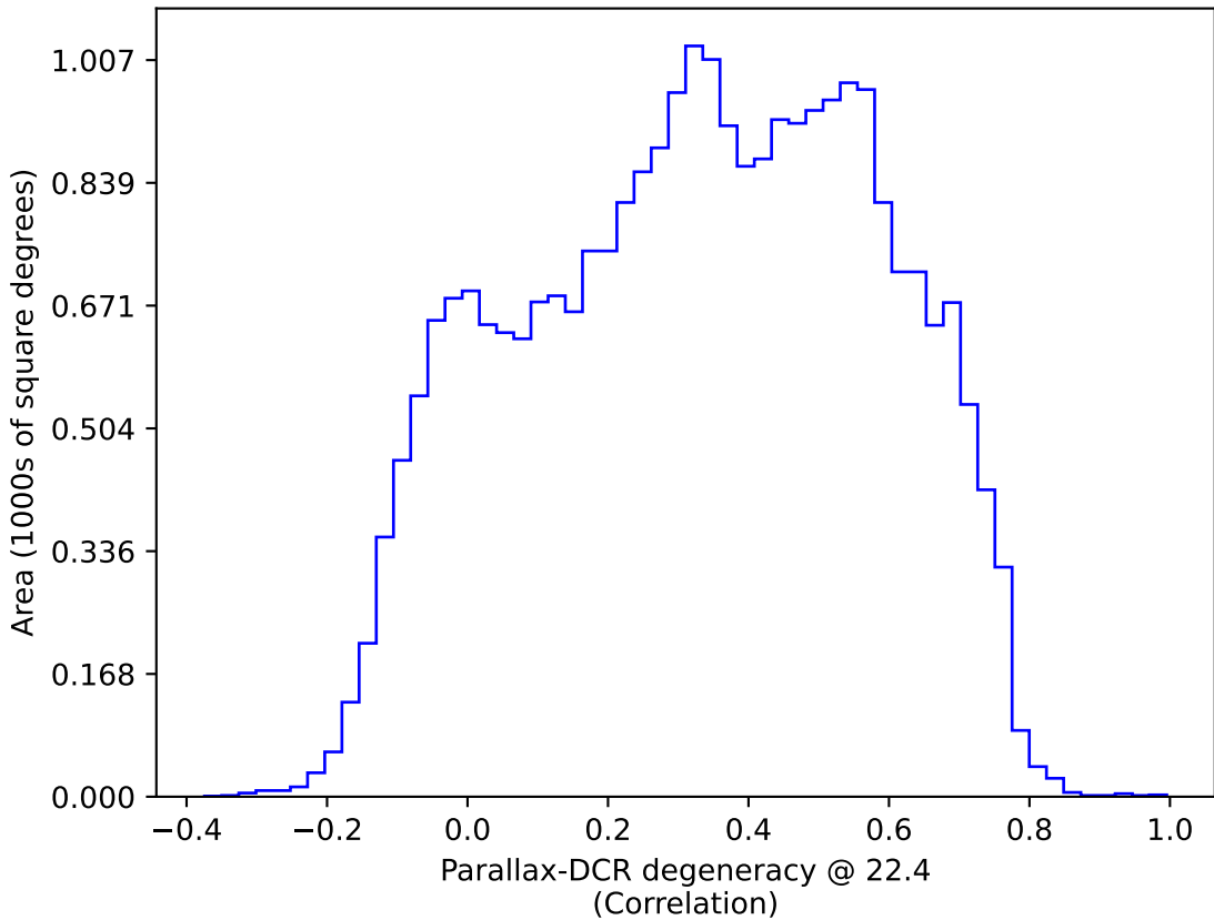
too_5_4v3.4_10yrs : Parallax-DCR degeneracy @ 22.4
