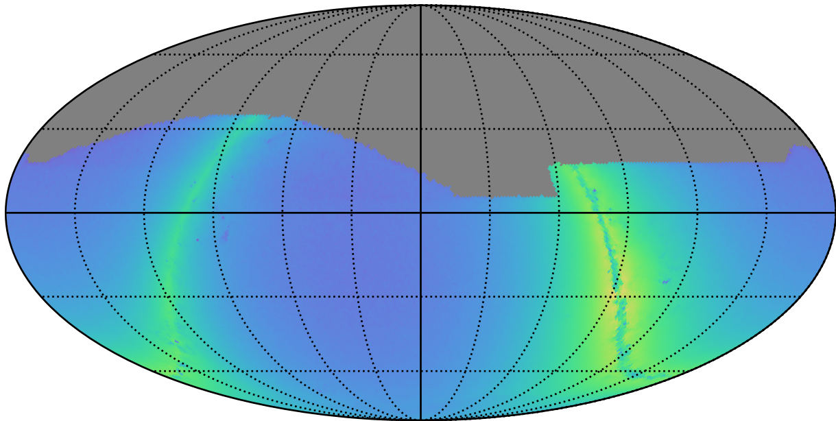
too_5_4v3.4_10yrs z: Nstars_no_crowding
