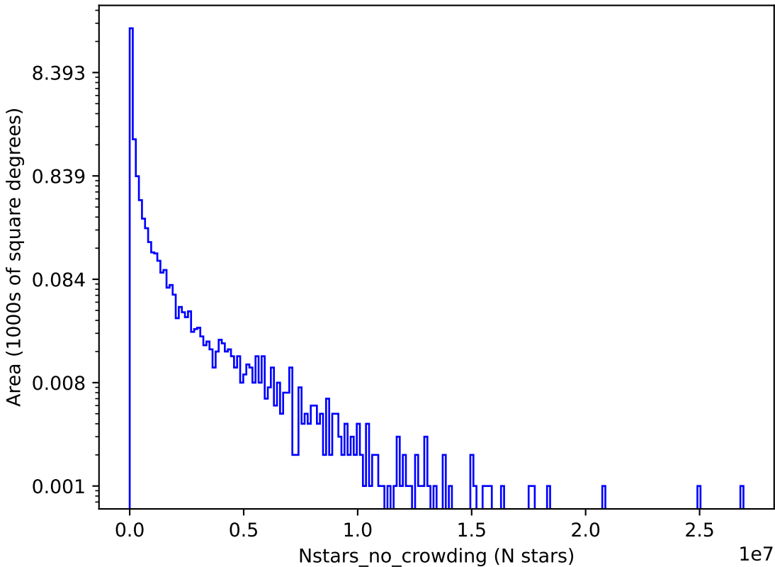
too_5_4v3.4_10yrs z: Nstars_no_crowding
