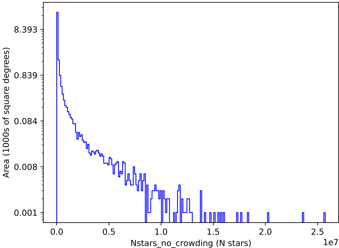
too_5_4v3.4_10yrs y: Nstars_no_crowding
