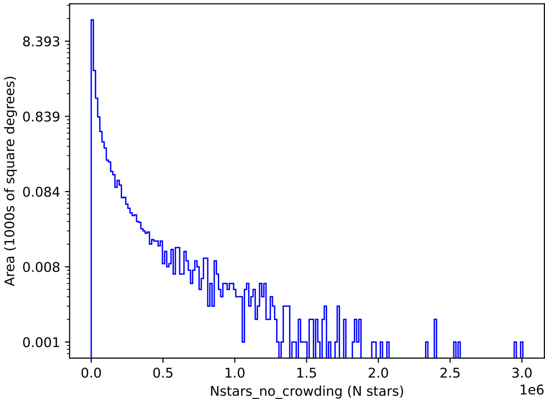
too_5_4v3.4_10yrs u: Nstars_no_crowding
