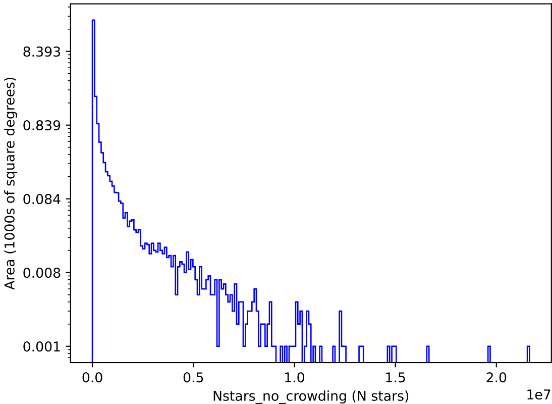
too_5_4v3.4_10yrs r: Nstars_no_crowding
