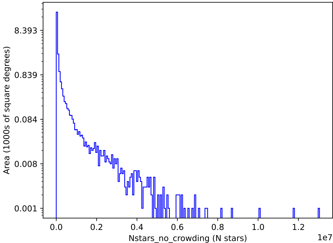
too_5_4v3.4_10yrs g: Nstars_no_crowding
