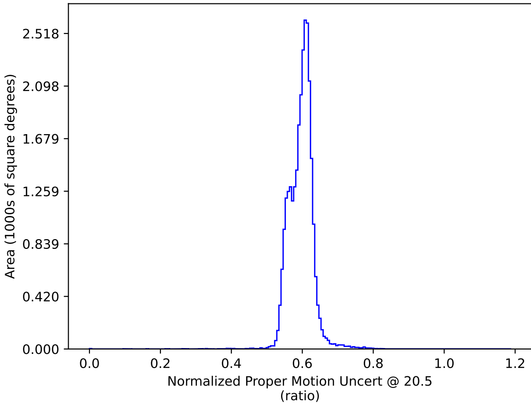
too_5_4v3.4_10yrs : Normalized Proper Motion Uncert @ 20.5
