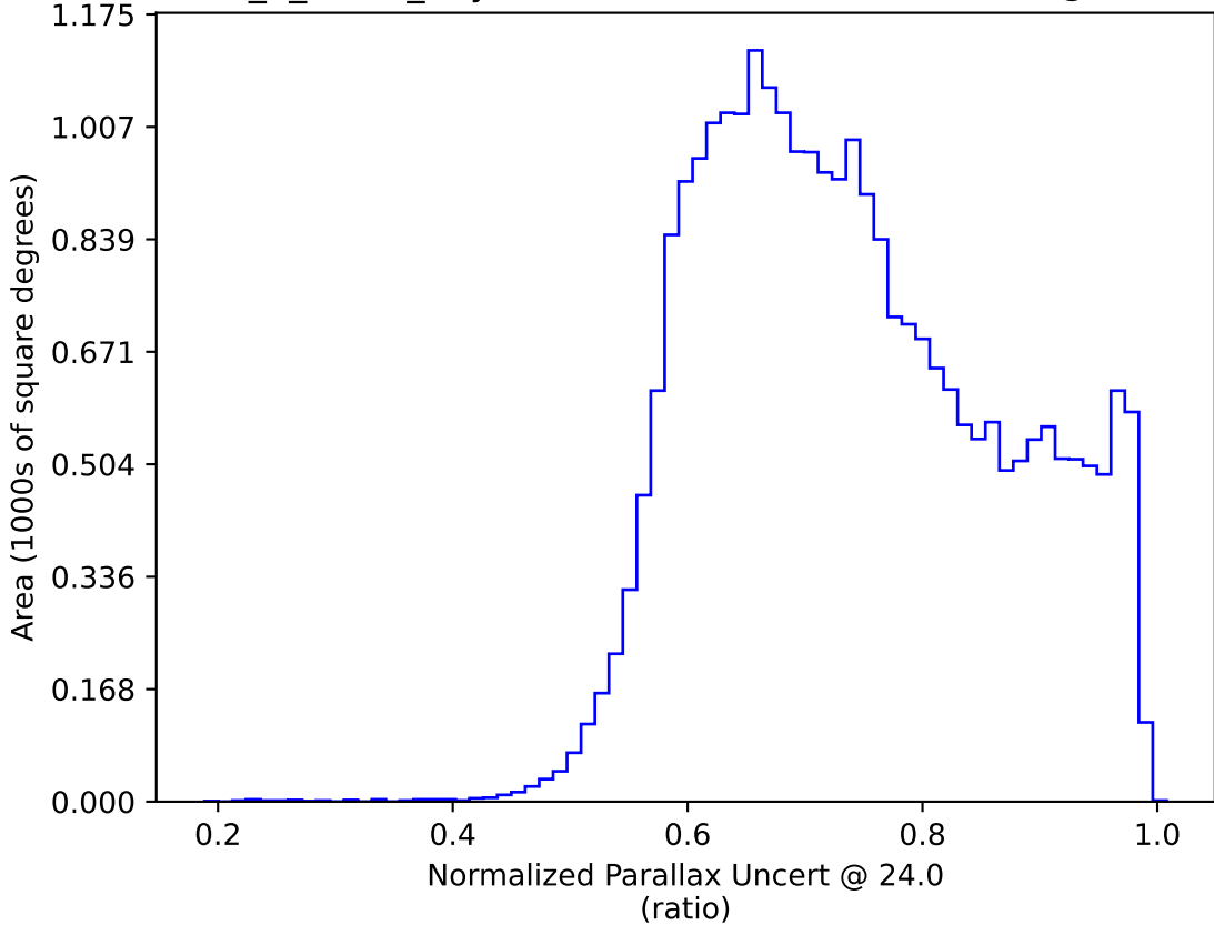
too_5_4v3.4_10yrs : Normalized Parallax Uncert @ 24.0
