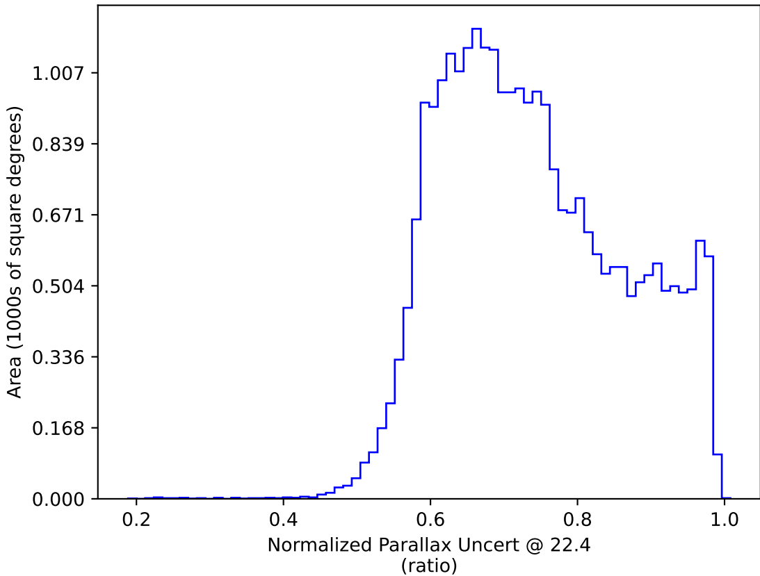
too_5_4v3.4_10yrs : Normalized Parallax Uncert @ 22.4
