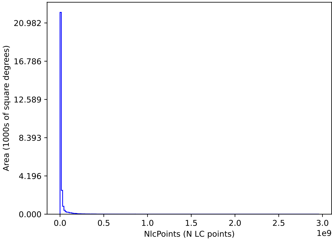
too_5_4v3.4_10yrs : NlcPoints
