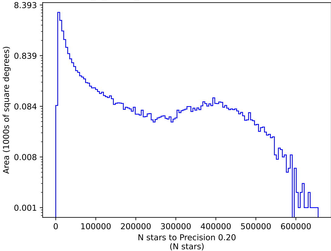
too_5_4v3.4_10yrs z: N stars to Precision 0.20
