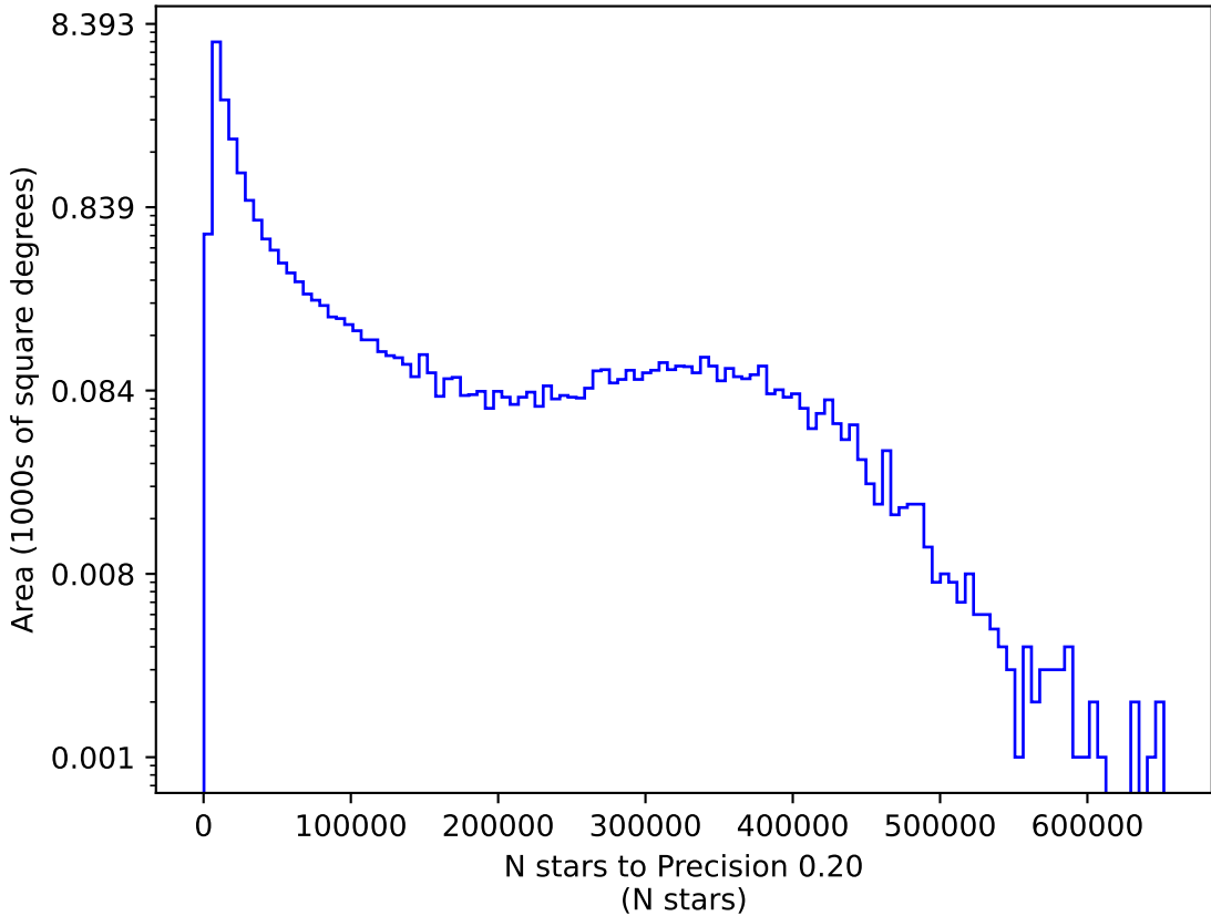
too_5_4v3.4_10yrs y: N stars to Precision 0.20
