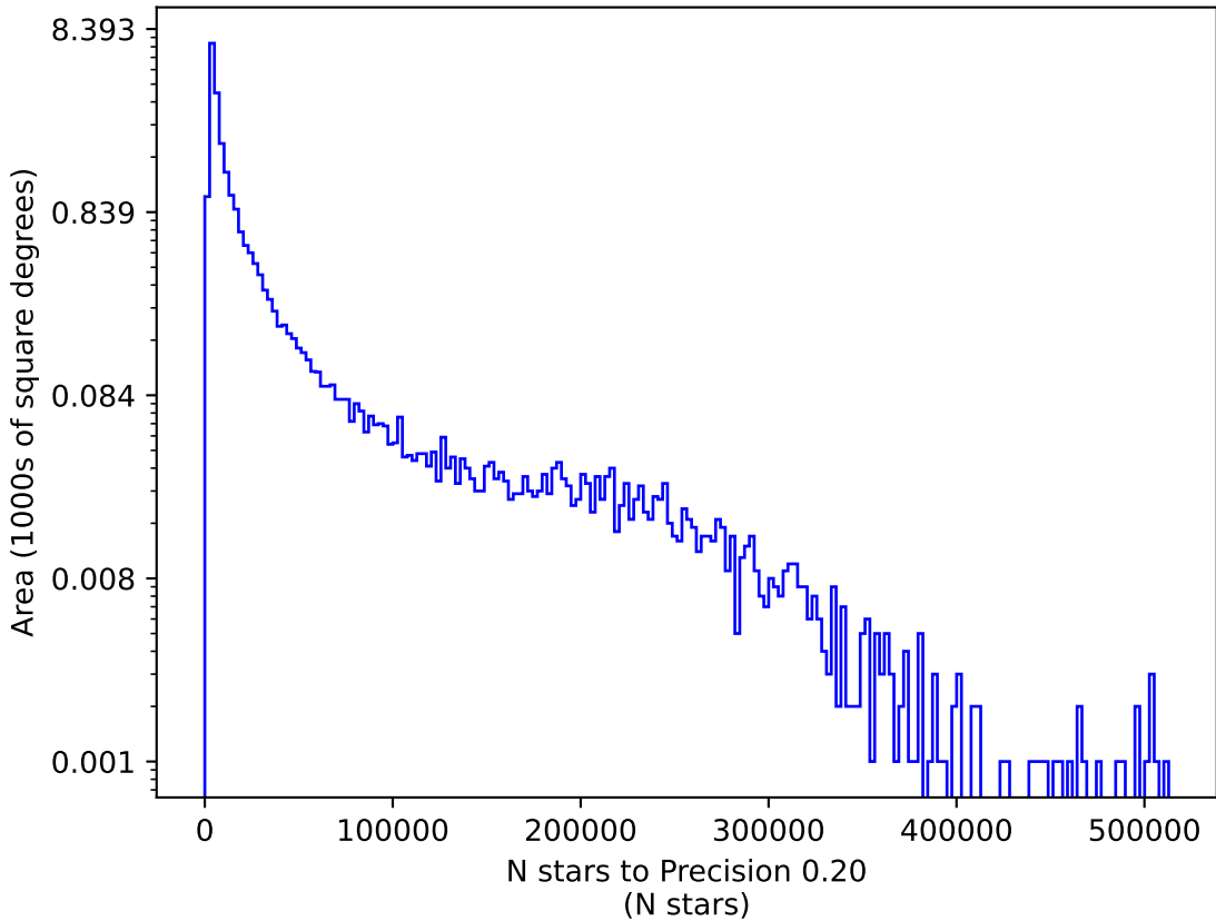
too_5_4v3.4_10yrs u: N stars to Precision 0.20
