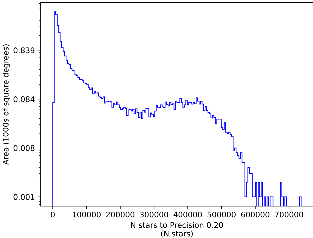
too_5_4v3.4_10yrs r: N stars to Precision 0.20
