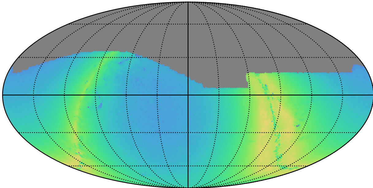
too_5_4v3.4_10yrs g: N stars to Precision 0.20
