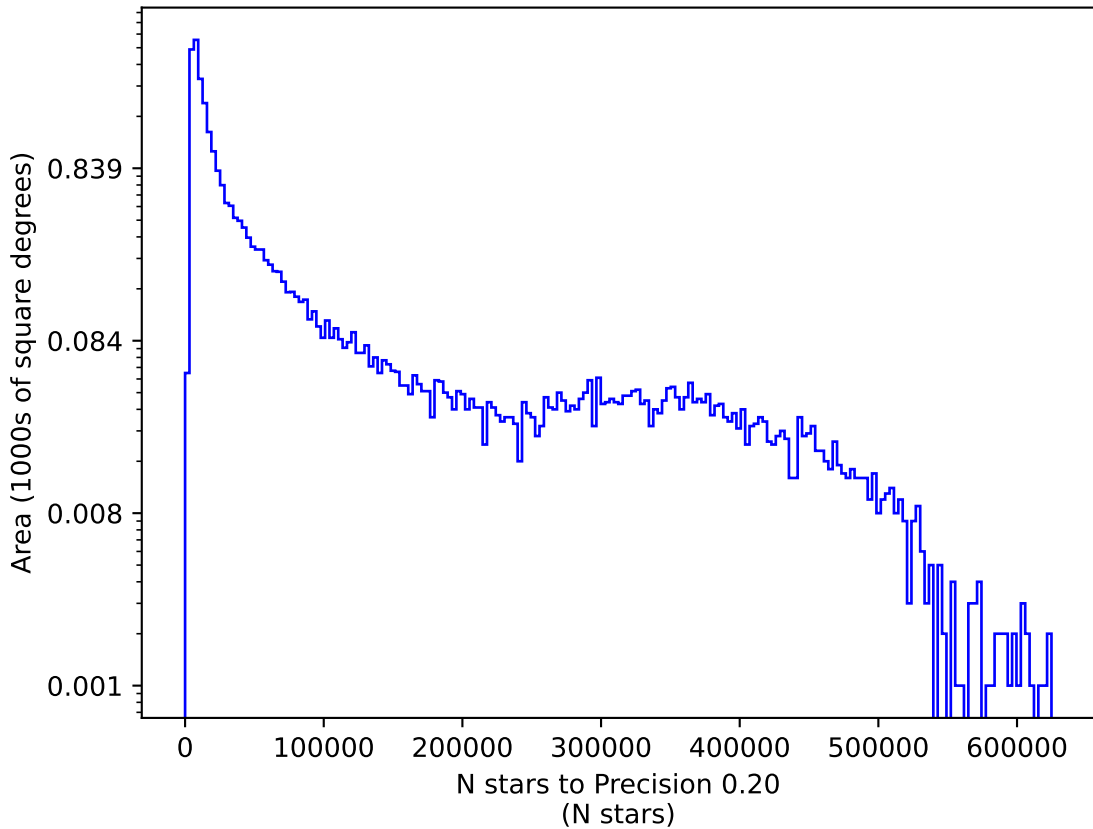
too_5_4v3.4_10yrs g: N stars to Precision 0.20
