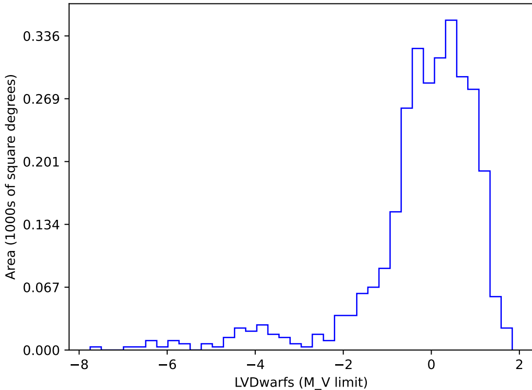
too_5_4v3.4_10yrs gi SCP: LVDwarfs
