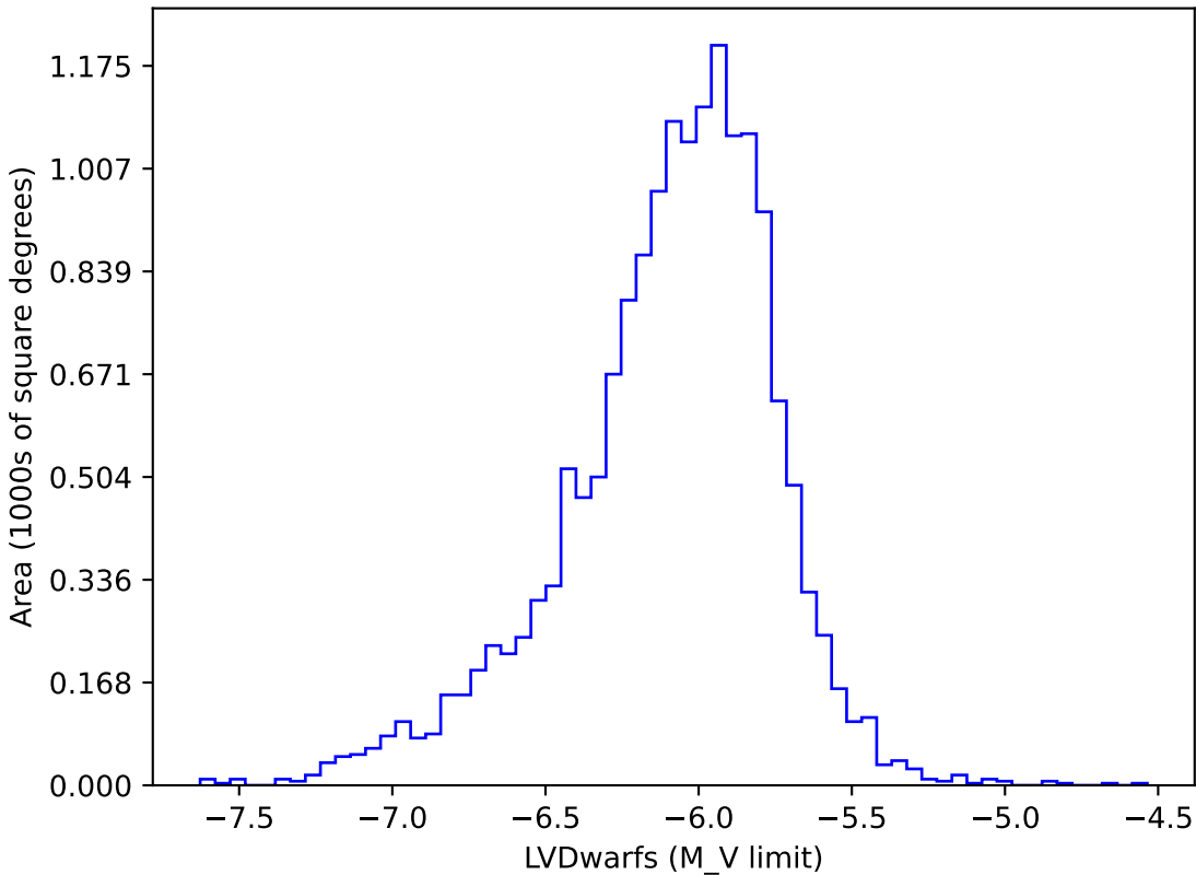
too_5_4v3.4_10yrs gi: LVDwarfs
