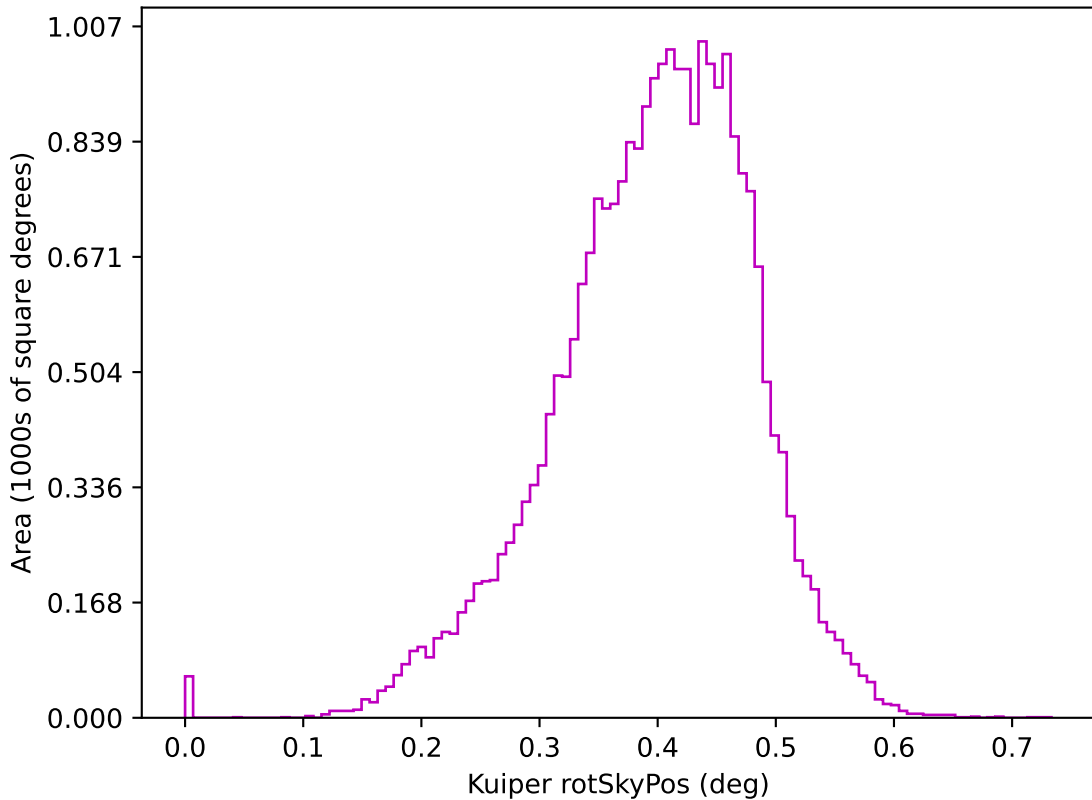
too_5_4v3.4_10yrs z: Kuiper rotSkyPos
