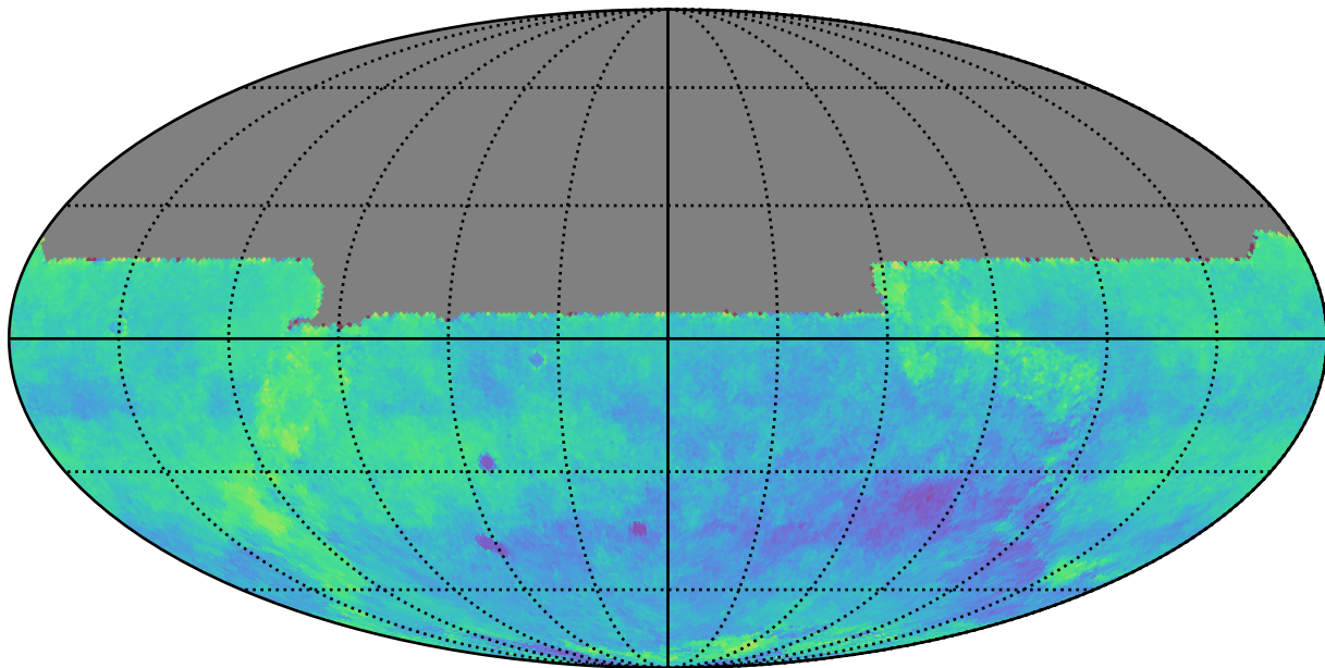
too_5_4v3.4_10yrs y: Kuiper rotSkyPos
