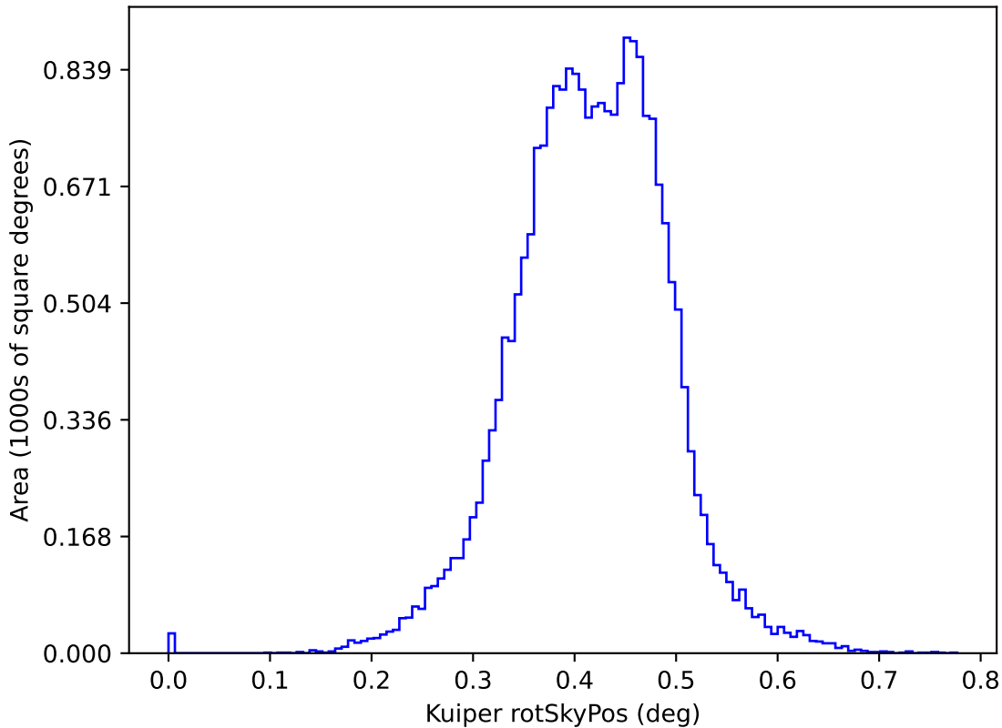
too_5_4v3.4_10yrs y: Kuiper rotSkyPos
